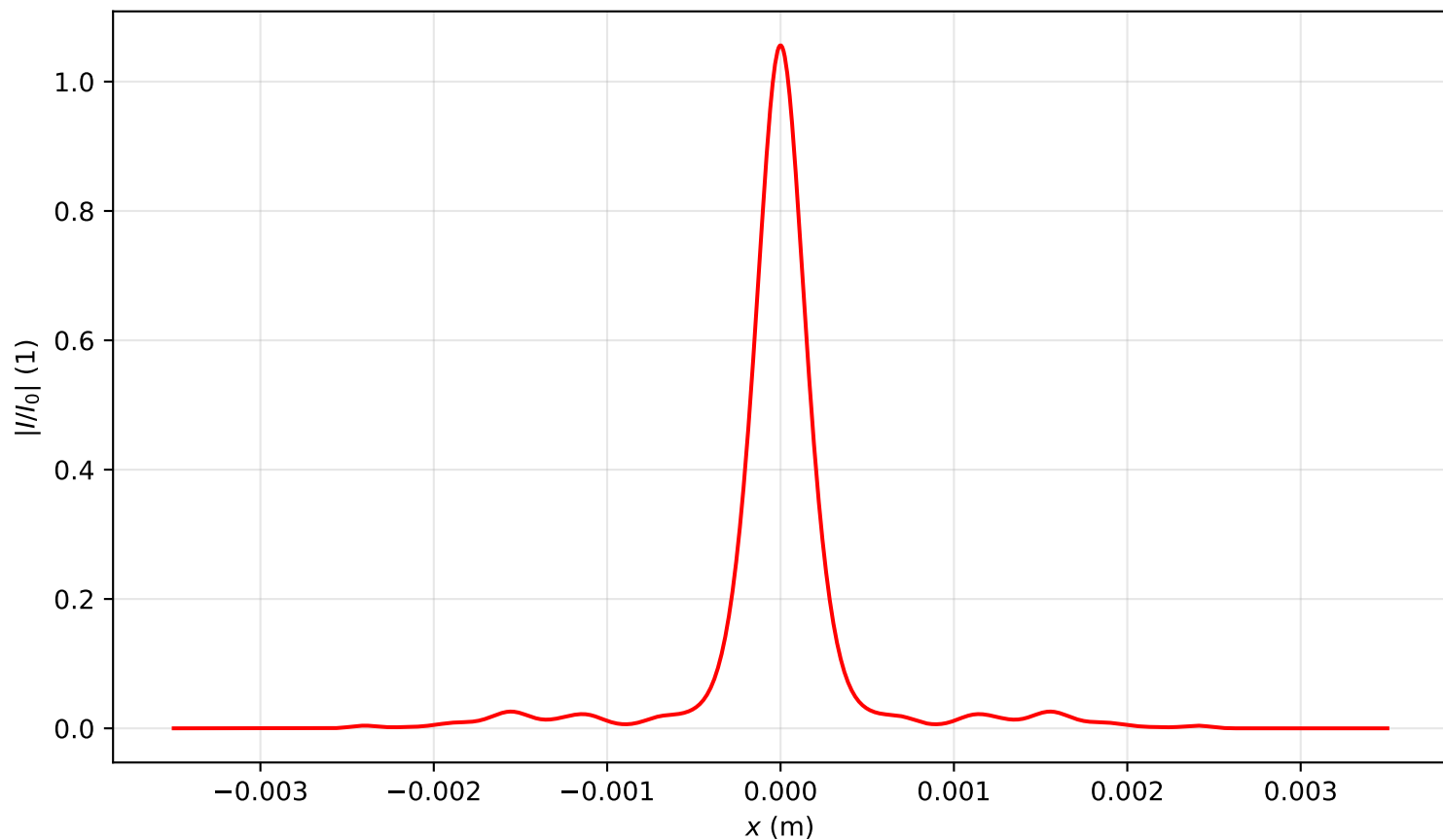
Intensity profile I(x, y = 0, z = 3.821)/I_0 , P_{in}=4.5P_{cr} , artificial time
